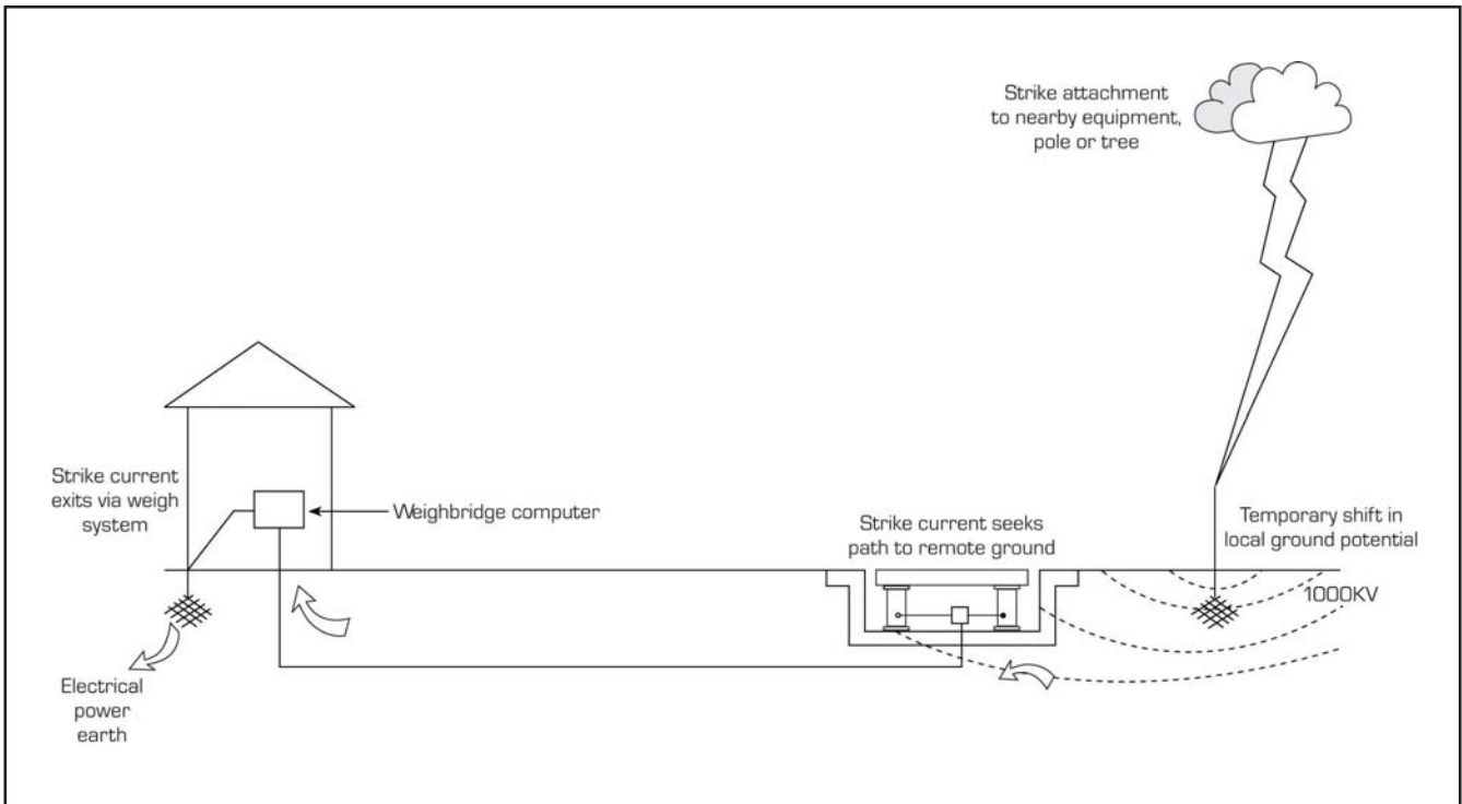
Figure 3 Weigh system damage caused by resistive coupling following a breakdown under local high voltage
