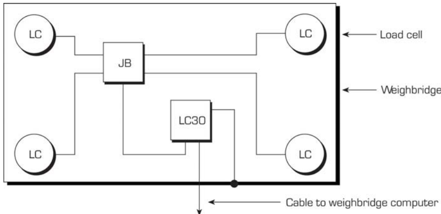
Figure 5 Weighbridge with field junction
