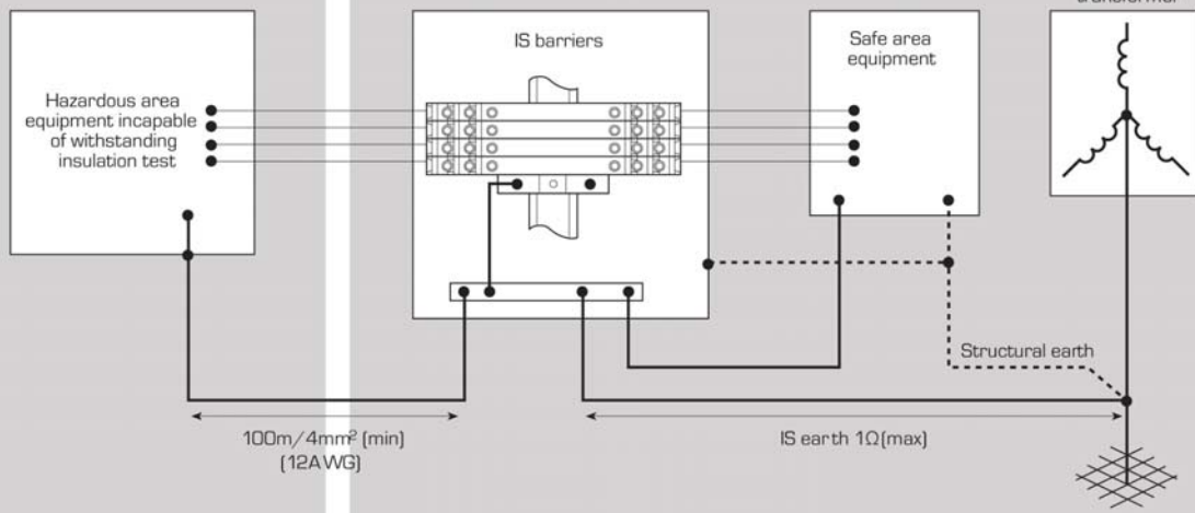
Figure 5 Potential equalizing conductors - UK practice
