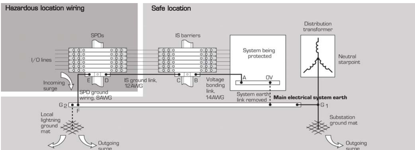
Figure 4 Recommended earthing system for loops including IS barriers and SPDs
